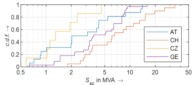
Fig. 2: Short circuit power of measurement sites by country.
