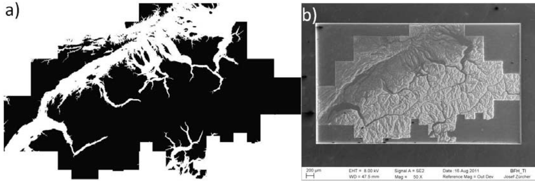
Figure 13: Structure based on topography data of Switzerland 19 a) typical black-and-white layer; b) SEM image of the structure, 120 mW, 300 kHz, 3 \mu m pitch, 447 layers
