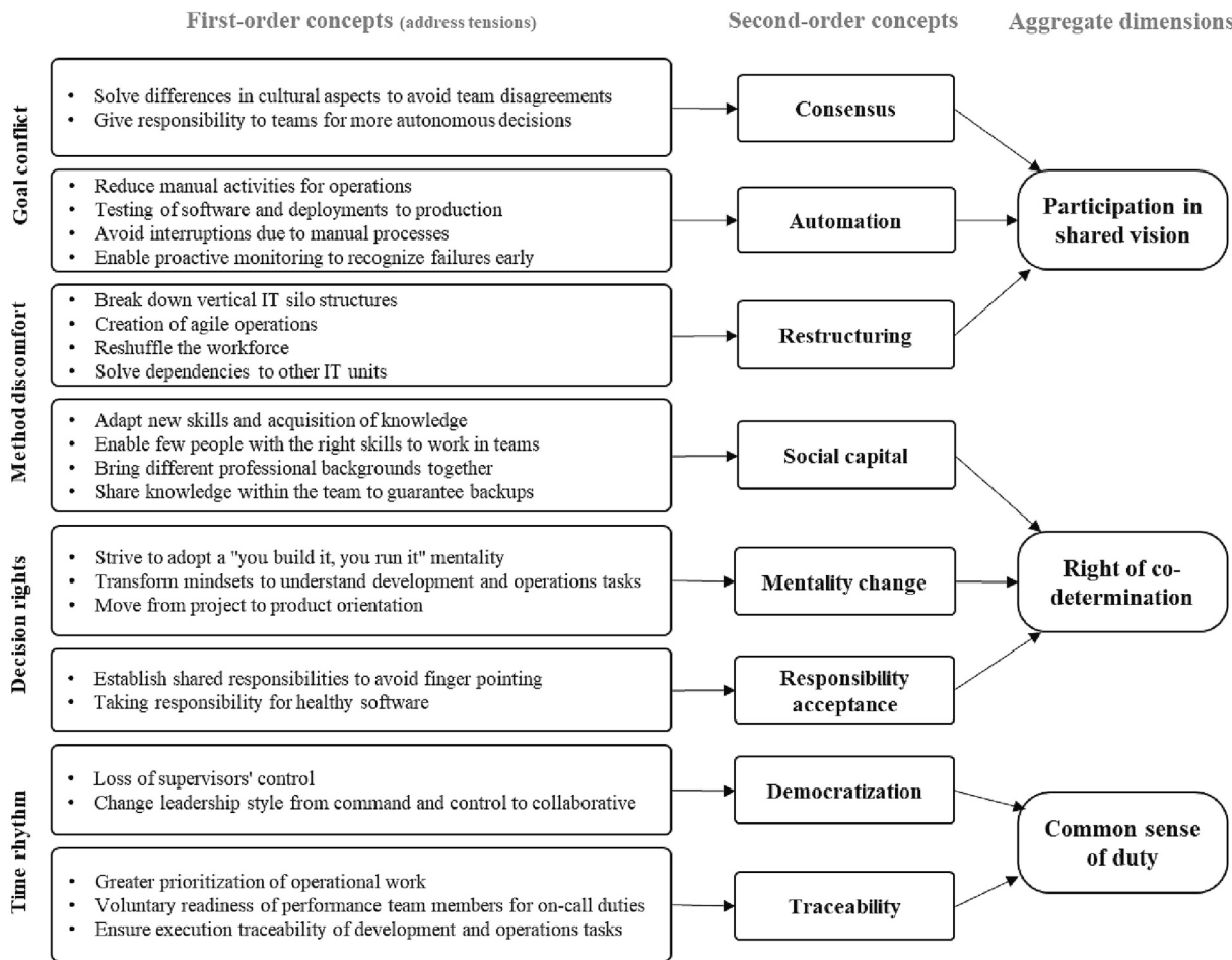
Fig. 1. Data structure.
