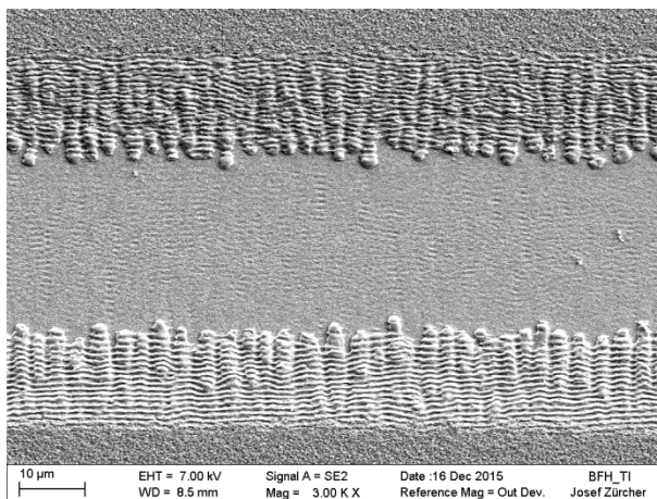
Figure 12 P2 scribe realized on rigid substrate (Mo/CIGS/IZO on glass; Empa). The laser used was Onefive Genki XP at around 4 W average power and a wavelength of 1064 nm. Achieved scribing velocity: 390 mm/s.
