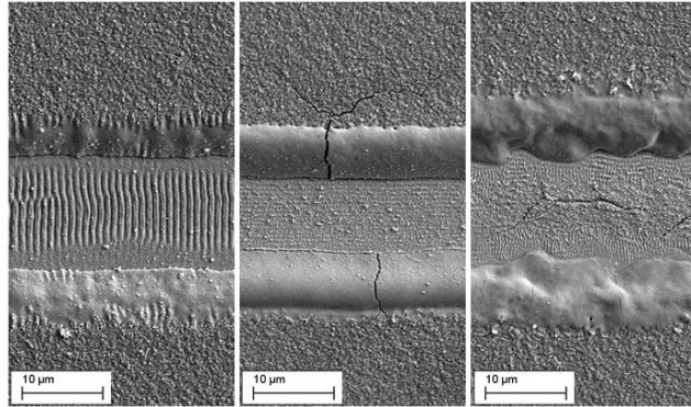
Figure 9 Three examples of often observed problems in P2 scribing (left to right): damage of the back contact layer (by strong ripple formation or ablation of the back contact), micro-cracks extending into the surrounding absorber material with beginning delamination of the layer stack, and cracks in the back contact in the direction of the scribe (thermal overload caused by heat accumulation).
