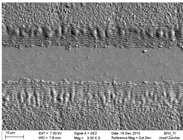
Figure 11 P2 scribe realized on flexible substrate (Mo/CIGS on PI substrate; Flisom). The laser used was Onefive Genki XP at 2.5 W average power and a wavelength of 1064 nm. Achieved scribing velocity: 380 mm/s.
