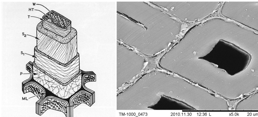
Figure 3: Left: Structure of a tracheid ( ML , middle lamella; P , primary wall; S1 , first layer of the secondary wall; S2 , second layer of the secondary wall; T , tertiary wall; HT , helical thickening; W , warty layer) [25] Right: Picea Abies : the primary, secondary and tertiary walls with the middle lamella are clearly visible (© wood anatomy laboratory Biel)
