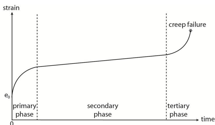
Figure 4: Definition of the three creep phases
