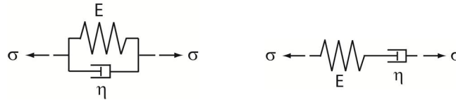
Figure 6: left: Schematic drawing of a Kelvin element right: Maxwell element
