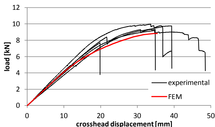
Figure 101: Load as a function of the crosshead displacement of the control specimens ( black: experimental measurements; red: FEM)
