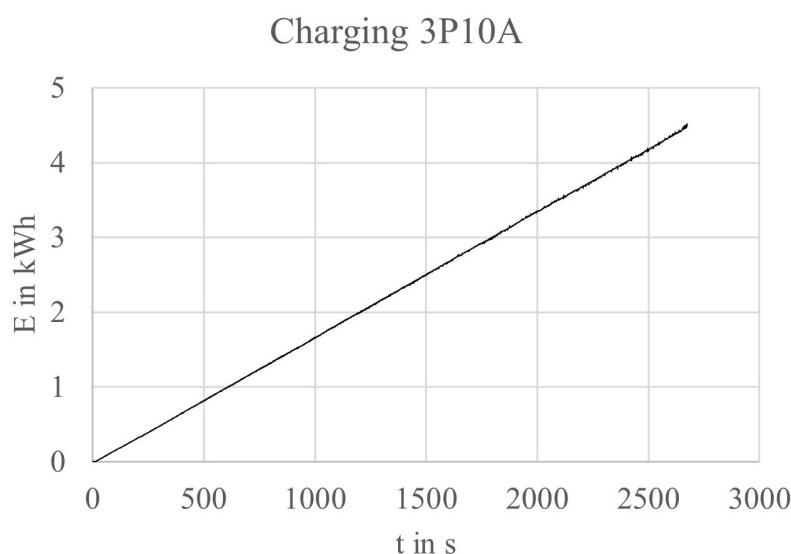
Figure 5. Accessed charged energy data after completing a WLTC.
