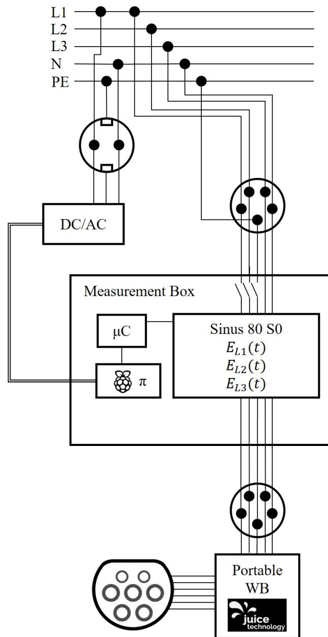
Figure 4. General overview measuring system.
