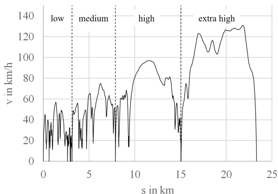
Figure 1. WLTC speed profile v as a function of the distance driven s (VW e-Up! data).
