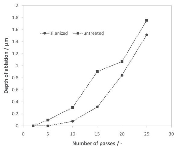
Figure 5: Depth of the ablation tracks as a function of the number of passes obtained with \text{CuSO}_4 as absorber for untreated (squares) and silanized (circles) soda lime glass surfaces. The dashed lines serve as guide to eye.
