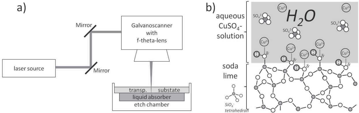
Figure 1: a) Experimental set-up for the LIBWE experiments; b) Schematic diagram of the physisorption of Cu 2+ ions at the polar soda lime surface.
