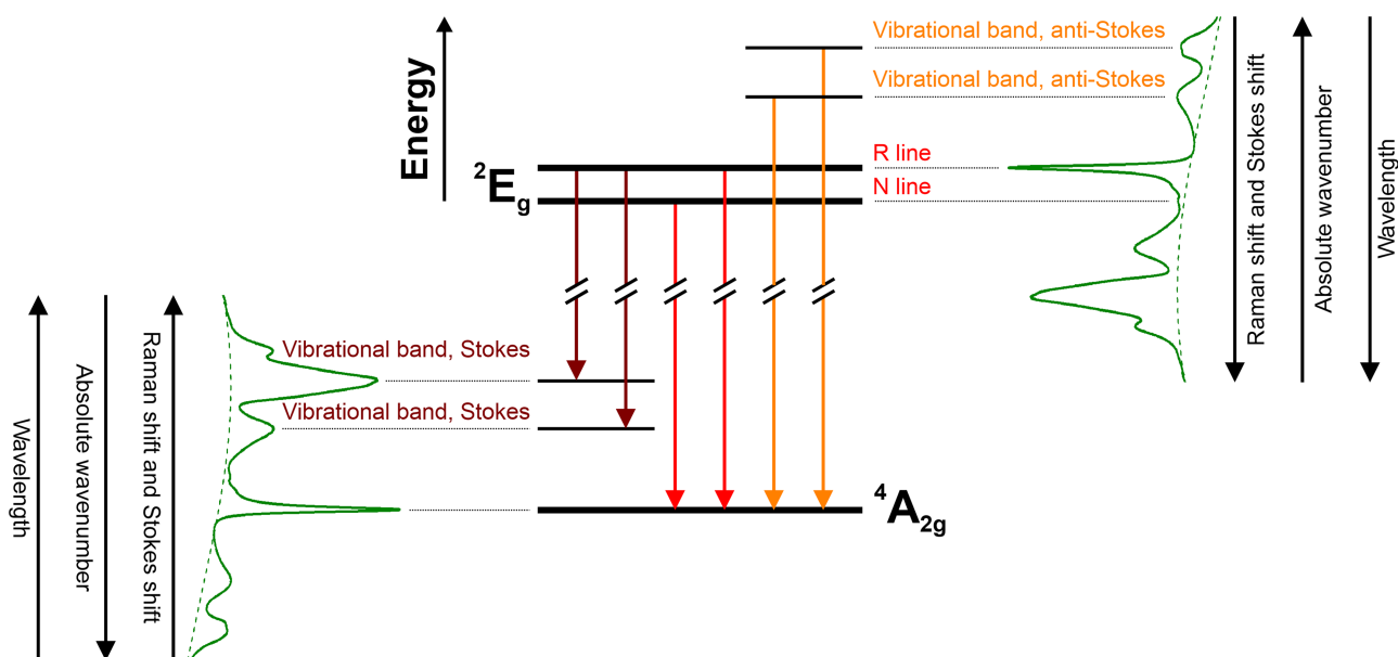
FIGURE 3 Schematic explanation of the sharp features in the red luminescence emission of MgO:Cr 3+ [Colour figure can be viewed at wileyonlinelibrary.com ]
