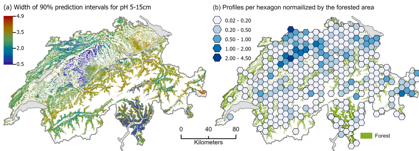
Fig. 8. Uncertainty map for the pH predicted for 5–15 cm soil depth (a) and aggregated density map of soil profiles (b). Uncertainty is based on the width of the 90% prediction intervals using quantile regression forest and is expressed in pH units. The aggregated density map reflects the number of calibration soil profiles per km 2 forested area within a hexagon (interhexagon distance is 10 km). If no hexagon is present, there were no calibration points within this area.
