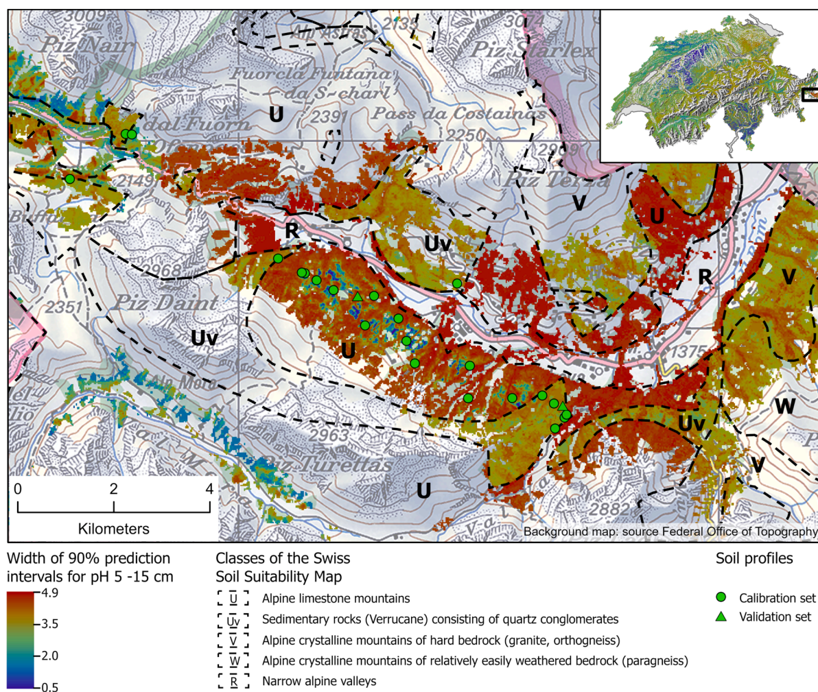
Fig. 9. Uncertainty map of pH (5–15 cm) for the Müntertal area. Within the class U of the Soil Suitability Map (Swiss Federal Statistical Office, 2001), the prediction interval and thus the uncertainty is higher than in the adjacent classes Uv and V.
