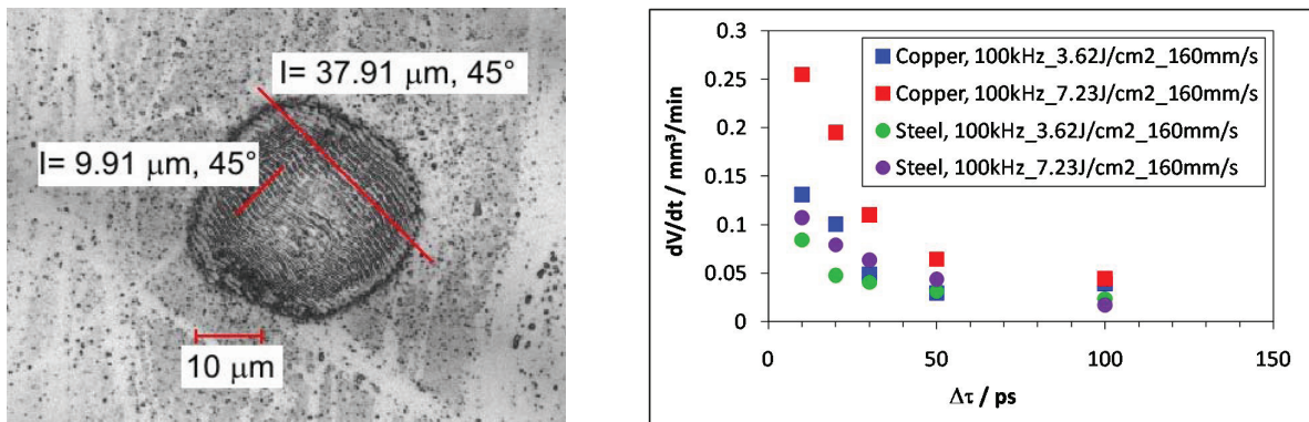
Figure 4. (a) Ripples orientation and distance in steel, 10 ps 1.45 J/cm 2 peak fluence 32 pulses; (b) Volume ablation rate at constant fluence versus pulse duration
