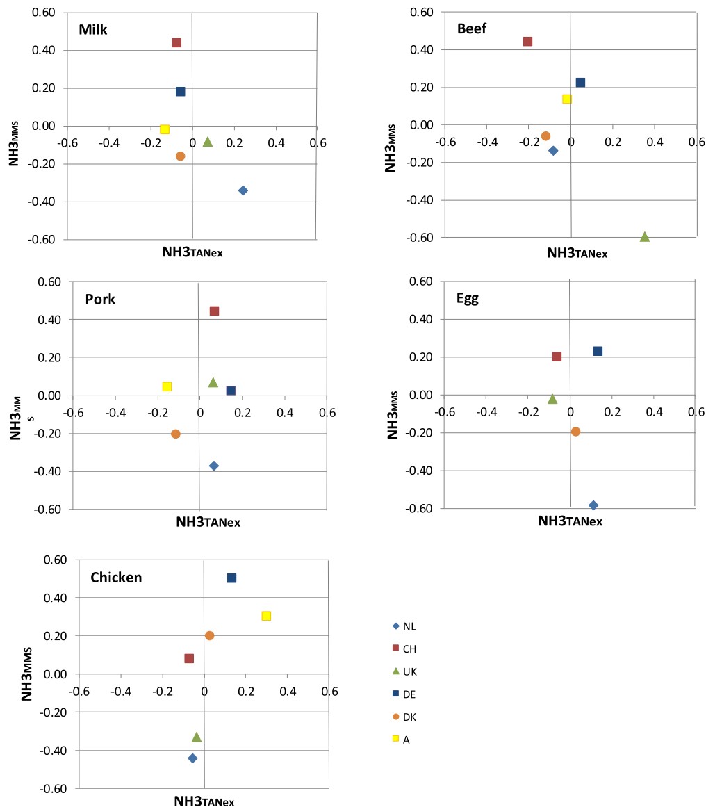
Fig. 4. Relative contribution of manure management (EF) to \text{NH}_3 ( \text{NH}_3_{\text{MMS}} ) versus that of TAN excretion ( \text{NH}_3_{\text{TANex}} ) for milk, beef, pork, eggs, and chicken in the six different countries NL (light blue), CH (red), UK (green), DE (dark blue), A (yellow), DK (orange); a: low TAN, high EF; b: high TAN, high EF; c: high TAN, low EF; d: low TAN, low EF. (For interpretation of the references to colour in this figure legend, the reader is referred to the Web version of this article.)
