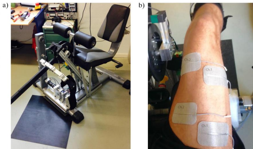
Fig 1. (a) The Knee Dynamometer designed to measure isokinetic knee joint torque. (b) Electrode setup on the right leg.
