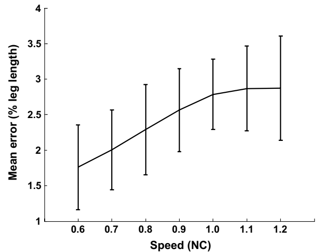
Fig. 4 Mean error between the best-fit circle and the relative toe trajectories from all subjects walking at seven speeds
