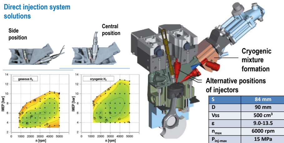
Fig. 15. Solutions for direct and indirect injection of hydrogen in an internal combustion engine [16]
