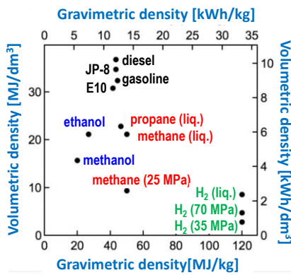
Fig. 7. Energy specifications for liquid and gaseous fuels (including hydrogen) [14]
