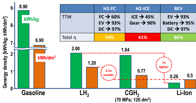
Fig. 11. Hydrogen vs. batteries in vehicle propulsion systems [18]
