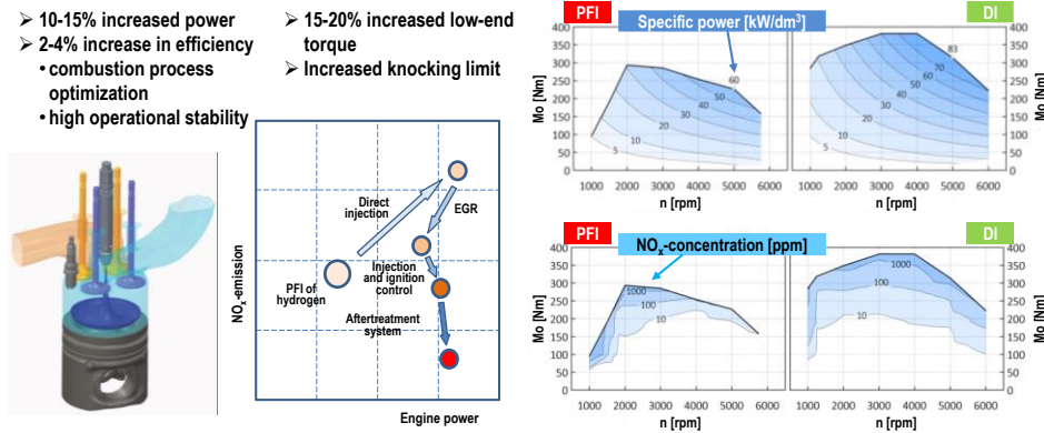
Fig. 18. Solutions for direct and indirect injection of hydrogen in a combustion engine [8, 28]
