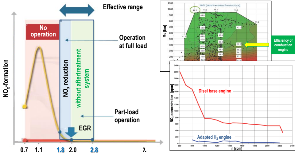
Fig. 16. Hydrogen injection and combustion in an internal combustion engine [33]
