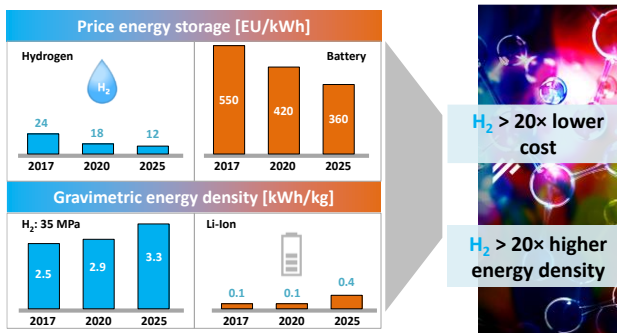
Fig. 1. Energy density of hydrogen and Li-Ion batteries [35]
