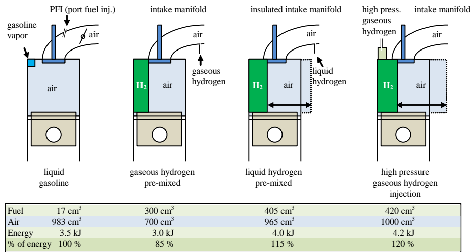
Fig. 13. Hydrogen injection systems for combustion engines [2, 4, 17]
