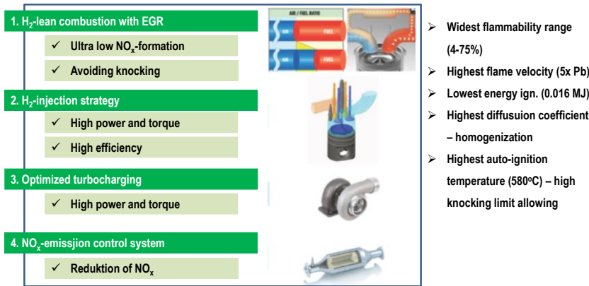
Fig. 17. Hydrogen combustion process in a combustion engine [33]
