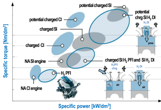
Fig. 12. Combustion engines concepts [17, 19]
