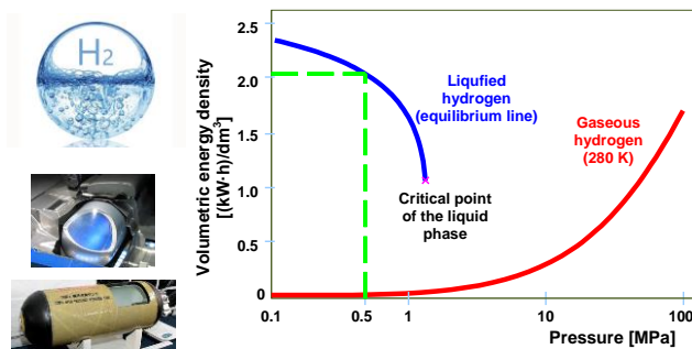
Fig. 5. Physical parameters of liquefied and compressed hydrogen [20]
