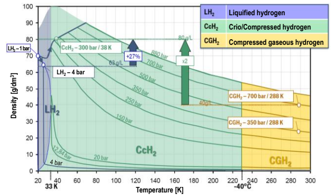
Fig. 8. Hydrogen storage conditions [5]
