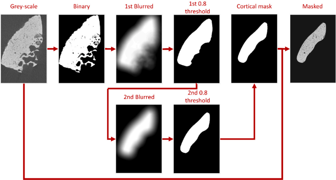
Fig. A1. Steps of the micro-CT image processing.
