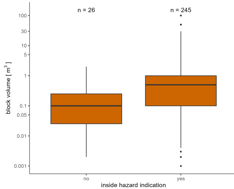
Figure 6. Distribution of block volumes in m 3 of PE from FL, distinguished according to whether they are located inside the generated HIZ or not (yes/no).
