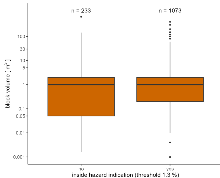
Figure 7. Distribution of block volumes in m 3 of PE from GR, distinguished according to whether they are located inside the generated HIZ delimited using a threshold of 1.3% or not (yes/no).
