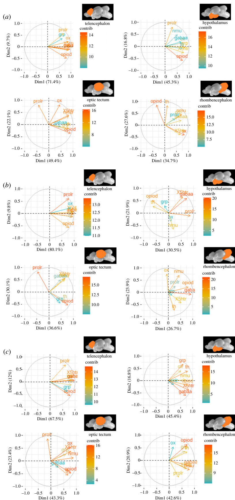
Figure 8. Quality of representation of the mRNA expression of ox , nmu , gaba a , prolr , opiod , 5htr , grp and th in fish 10 (a), 30 (b) and 60 min (c) after treatment on the factor map \cos^2 (the numbers next to Dim1 and Dim2 indicate the percentage of the variance in the datasets that is explained by the first two components of the PCA), n = 6 per treatment.
