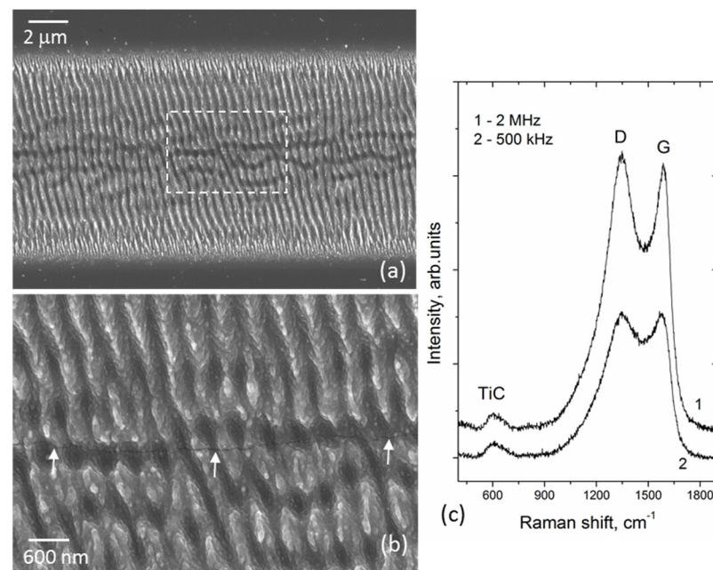
Figure 4. (a) SEM image of a microgroove formed on the 18%Ti-DLN film at f = 2 MHz, \varepsilon_p = 0.25 \mu\text{J} and V_s = 1 m/s ( E \parallel V_s ); (b) SEM image of a marked area in the groove center, with the arrows indicating the crack formation along the groove bottom; (c) Raman spectra of the microgrooves formed at f = 2 MHz and f = 500 kHz.
