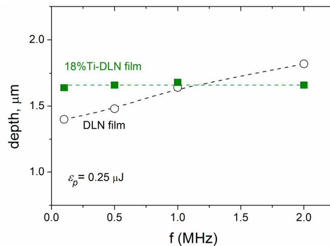
Figure 3. Influence of the pulse frequency on the ablation depth of microgrooves formed on the Ti-DLN film at the identical parameters of the pulse energy \varepsilon_p = 0.25 \mu\text{J} and effective pulse number N_{eff} = 2w_0 / (V_s/f) , compared to the ablation depth vs. pulse frequency for the DLN film ( E \parallel V_s ).
