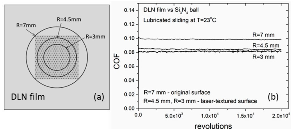
Figure 6. (a) Schematic of the friction measurements on the laser-textured DLN film, and (b) lubricated friction performance of the original film ( R = 7 \text{mm} ) and laser-textured ( R = 4.5 \text{mm} and R = 3 \text{mm} ) surface at T = 23 ^\circ\text{C} ; load 1 N, sliding speed 5 \text{cm/s} .
