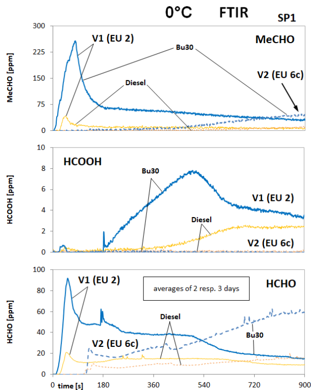
Fig. 13. Comparison of non-legislated gaseous exhaust emissions during cold start at 0°C and idling with different fuels, V1 & V2
