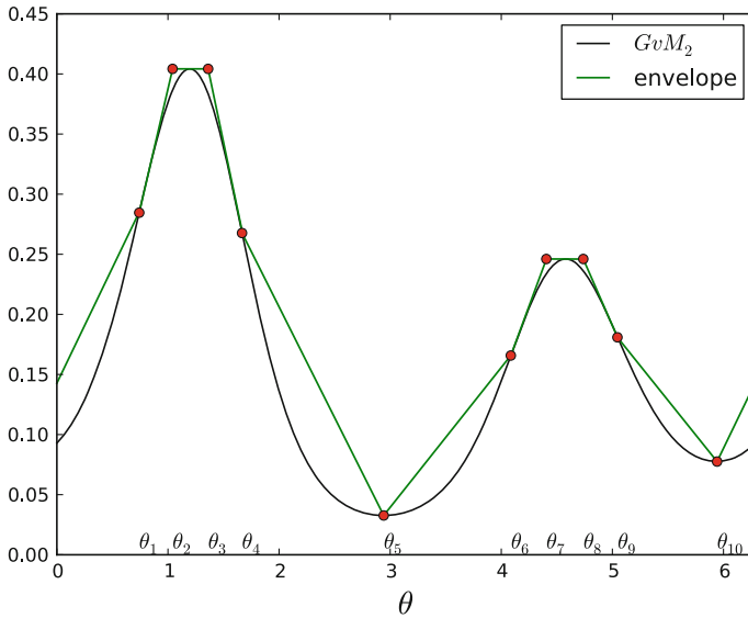
Fig. 1 The GvM(15°, 75°, 0.5, 0.9) density with the corresponding piecewise linear envelope
